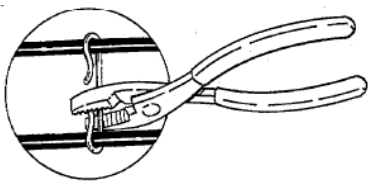
Figure 18. Squeezing spacers with pliers
