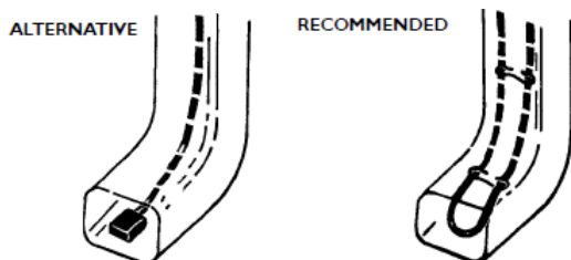
Figure 22. Cable in “end of run” downspouts
