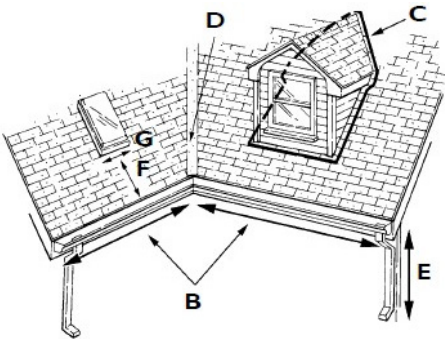
Figure B-3. Roof Measurements
