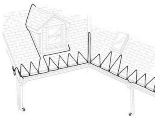
Figure 3. Typical pattern along roofline and in gutters/Downspouts
