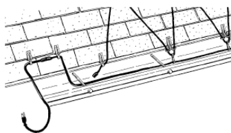
Figure 11. Starting point along gutter edge
