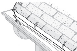
Figure 20b. Double run of cable in gutter-only applications (gutters without gutter spikes)
