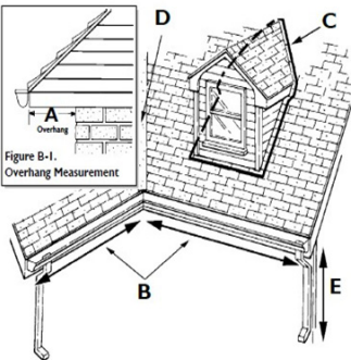
Figure B-2. Roof Measurements
